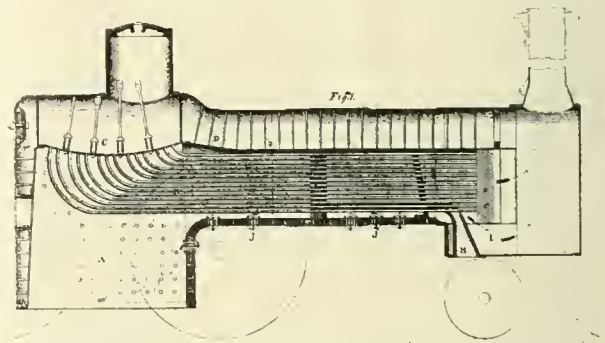
DIMPFEL'S COAL BURNING BOILER. FIG. 70.
